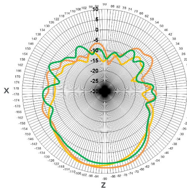
H Plane
