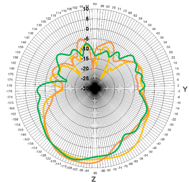
E Plane
