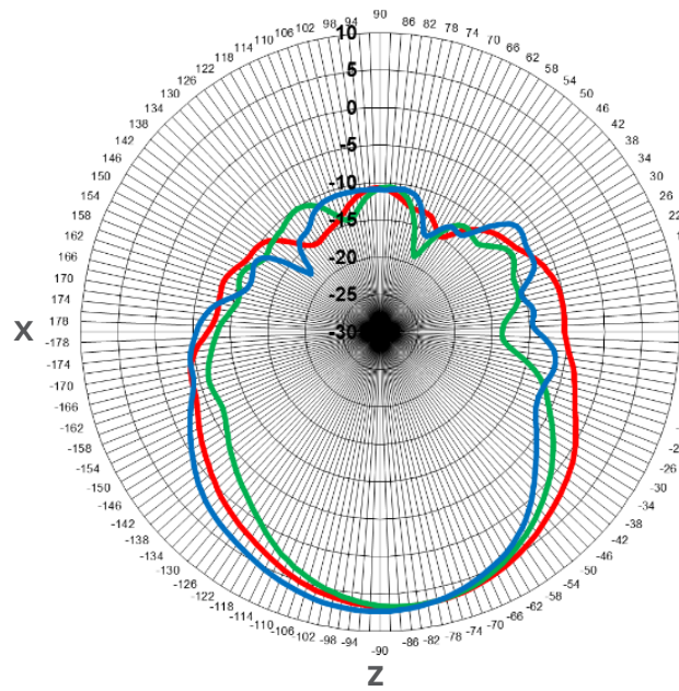
H Plane
