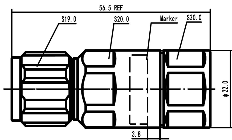
NM-LCF12-C03 Outline Drawing
