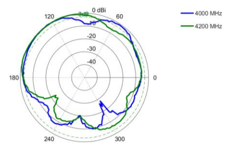
Elevation 2: 4000 – 4200 MHz
