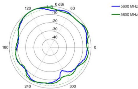
Elevation 2: 5600 – 5800 MHz
