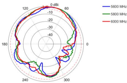
Elevation 2: 5600 – 6000 MHz
