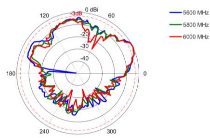
Elevation 2: 5600 – 6000 MHz
