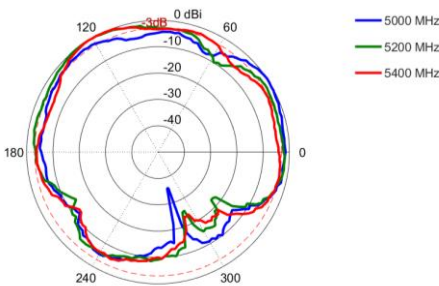
Azimuth: 5000 – 5400 MHz
