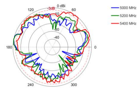
Elevation 1: 5000 – 5400 MHz
