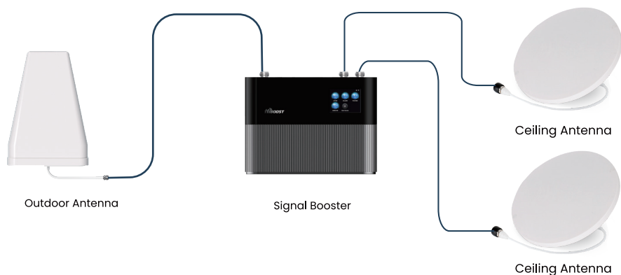
Figure 4 — Correct booster cable routing. Outdoor antenna to OUT; Indoor antenna to IN.
